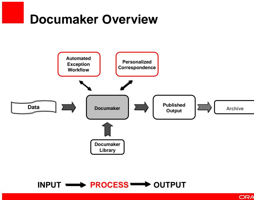
Figure 3: Documaker Overview
